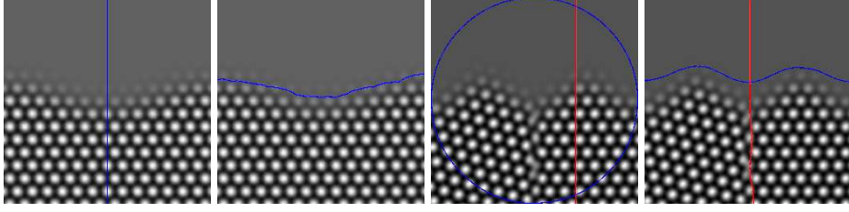
Fig. 4. Liquid-solid interface detection on artificial test data: input image u (first picture) with initial zero level set of \phi and computed interface (second picture). Combined grain boundary and liquid-solid interface detection on artificial test data: input image u (third picture) with the initial grain boundary in red and the initial liquid-solid interface in blue, final grain boundary and liquid-solid interface location (fourth picture).
