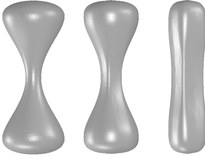
Fig. 5. From left to right the initial surface and two evolution steps of an anisotropic mean curvature flow are depicted (graphically scaled).
