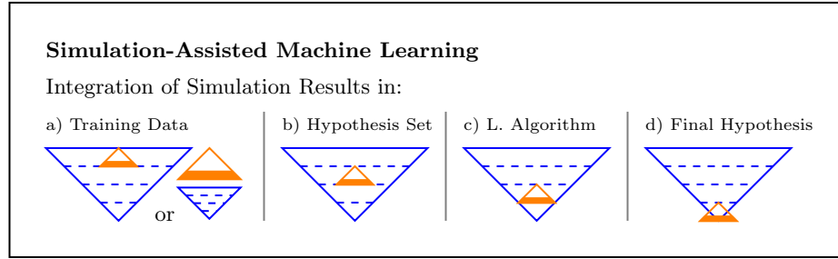
Fig. 4. Types of Simulation-Assisted Machine Learning. Simulations, in particular the simulation results, can be generally integrated into the four different components of machine learning. The triangles illustrate the machine learning (blue / dark gray) or the simulation (orange / light gray) approach and their components, which are themselves presented in Figures 2 and 3. The simulation results can be used to a) augment the training data, b) define parts of the hypothesis set in the form of empirical functions, c) steer the training algorithm in generative adversarial networks, or d) verify the final hypothesis against scientific consistency.
