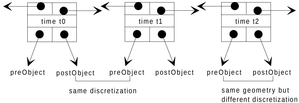
Figure 2: The Class TimeStep
