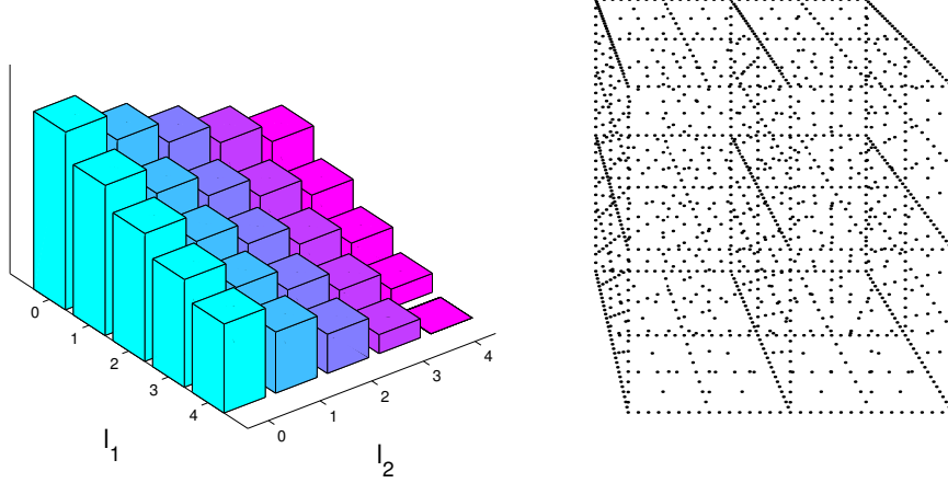
FIGURE 1. Left: Norms of errors of the difference spaces W_{\underline{l}} on a logarithmic scale. The example function is u(x_1, x_2) = e^{-(x_1^2 + x_2^2)} with (x_1, x_2) \in [0, 1] \times [0, 1] . Right: Sparse grid of refinement level l = 5 in three dimensions
