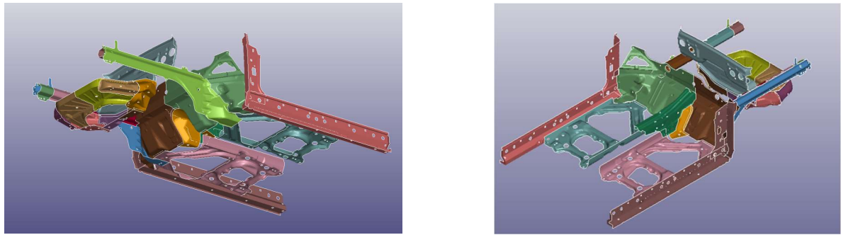
Figure 7 Parts (PIDs) of the car selected for the analysis of Global events.
