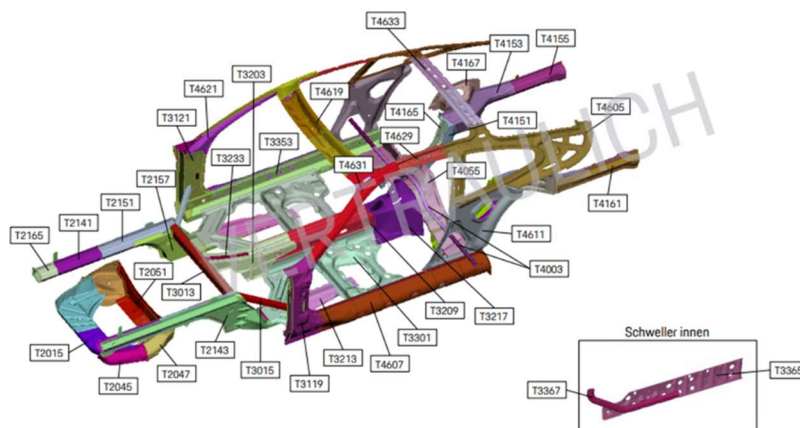
Figure 3 Structural members with thickness changes as considered in this study.
