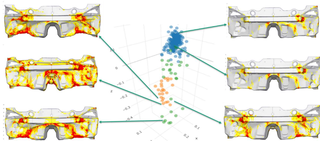
Figure 9 Example of an explorative analysis of the firewall, where the plastic strain at time step 27 is investigated. Note that the shown static two-dimensional picture of the three dimensional interactive visualization is limited. For example, the outlier on the bottom right appears close to the orange cluster, while it is actually further away, which one be seen by interactively rotating the three-dimensional visualization.
